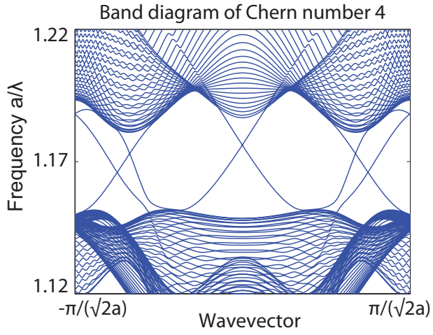
FIG. 3. The complete bandstructure for a metal-terminated supercell of the C_{gap} = 4 photonic crystal from Fig. 2 of the main text. This edge waveguide is oriented along the \Gamma - K direction. Unlike the other bandstructure plots in this letter, here we did not shade the bulk bands and we kept the edge modes from both ends of the supercell. This illustrates the connectivity between the bulk and edge bands.
