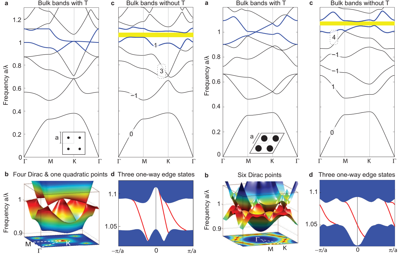
FIG. 1. Bulk and edge TM bandstructures showing three one-way edge states ( C_{gap} = 3 ) obtained from four Dirac points and one quadratic point. The photonic crystal is a square lattice of rods with a radius of 0.10a , \epsilon = 15 and \mu = 1 . The T-breaking perturbation corresponds to adding \mu_{12} = -\mu_{21} = 0.45i to the rods. a) Bulk bandstructure showing the Dirac point along \Gamma - K and quadratic point at K . The lower inset illustrates the lattice geometry. b) Four Dirac cones and one quadratic point between the 5th and 6th bands plotted in the whole Brillouin zone. c) Bulk bandstructure under T-breaking perturbation opens a 3.6% complete gap highlighted in yellow. Each band is labeled with its Chern number. The Chern number of degenerate bands is circled by a dotted line. d) Three gapless one-way edge states (red) appear in the projected edge band diagram when the bulk is terminated by a metallic boundary.
