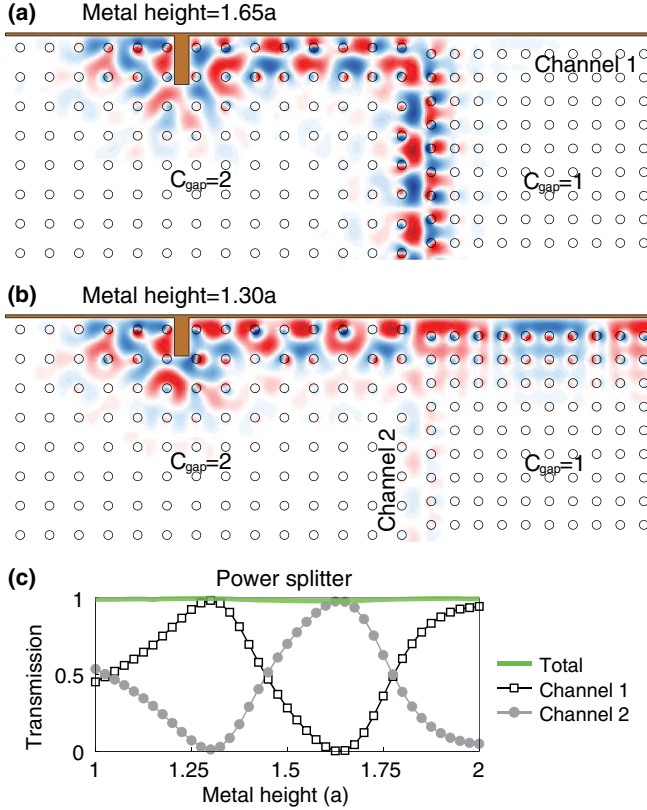
FIG. 4 (color online). A power splitter implemented with C_{\text{gap}} = 2 and C_{\text{gap}} = 1 gyromagnetic photonic crystals bordered on the top by a metallic wall. A point source with frequency a/\lambda = 0.82 couples light into the multimode waveguide to the left of the metal scatterer. The unit cell size of the C_{\text{gap}} = 2 lattice is a , the unit cell size of the C_{\text{gap}} = 1 lattice is 0.805a , and the rod radius for both lattices is 0.15a . The operating parameters are the same as in Fig. 3, so a in real units is 1.7 cm. (a) For a metal scatterer with height 1.65a , the majority of the light proceeds through channel 2 (bottom waveguide). (b) For a metal scatterer with height 1.30a , the majority of the light proceeds through channel 1 (right waveguide). (c) The transmission to each waveguide as a function of metal scatterer height.
