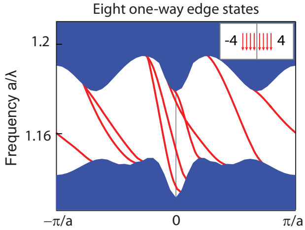
FIG. 4. An example of eight one-way edge states constructed by photonic crystals of opposite gap Chern numbers ( C_{gap} = \pm 4 ). We used the gyromagnetic photonic crystals of C_{gap} = 4 in Fig. 2 in the main text of this letter. Across the interface, the static magnetic field is reversed to get opposite Chern numbers.
